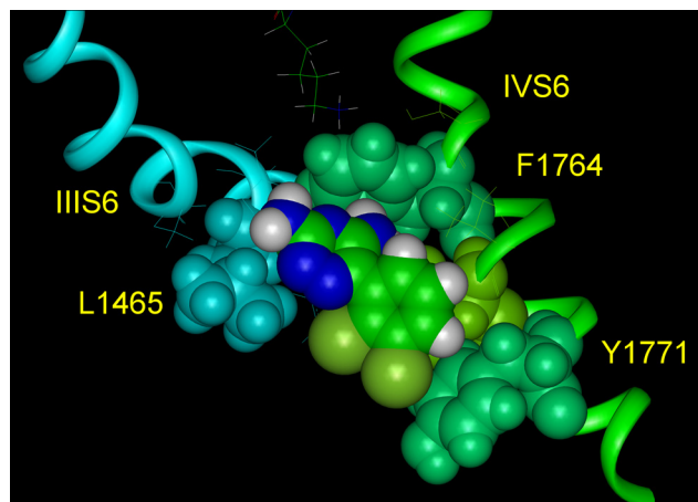
Fig. 9. Lamotrigine. Optimal location of lamotrigine inside the inner pore (side view). In accordance with the common pharmacophore core of anticonvulsants, the amino group in the 5-position of the triazine ring interacts with Phe-1764.
