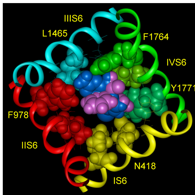
Fig. 10. Superposition of structures of carbamazepine (pink color) and lamotrigine (blue color) inside of the inner pore (top view). Different bulky anticonvulsants interact with the common receptor of the Na^+ channel and extend into the lumen of the pore in such a way that they could block conductance.
