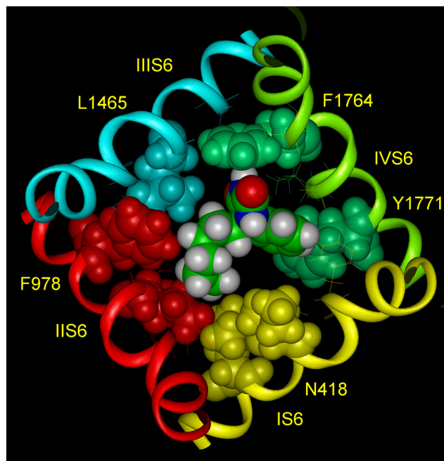
Fig. 5. 5-Hexyl-5-phenyl-hydantoin inside the inner pore (top view). The 5-hexyl alkyl chain participates in hydrophobic interactions with the nonpolar side chains of IS6–IIS6 helices.
